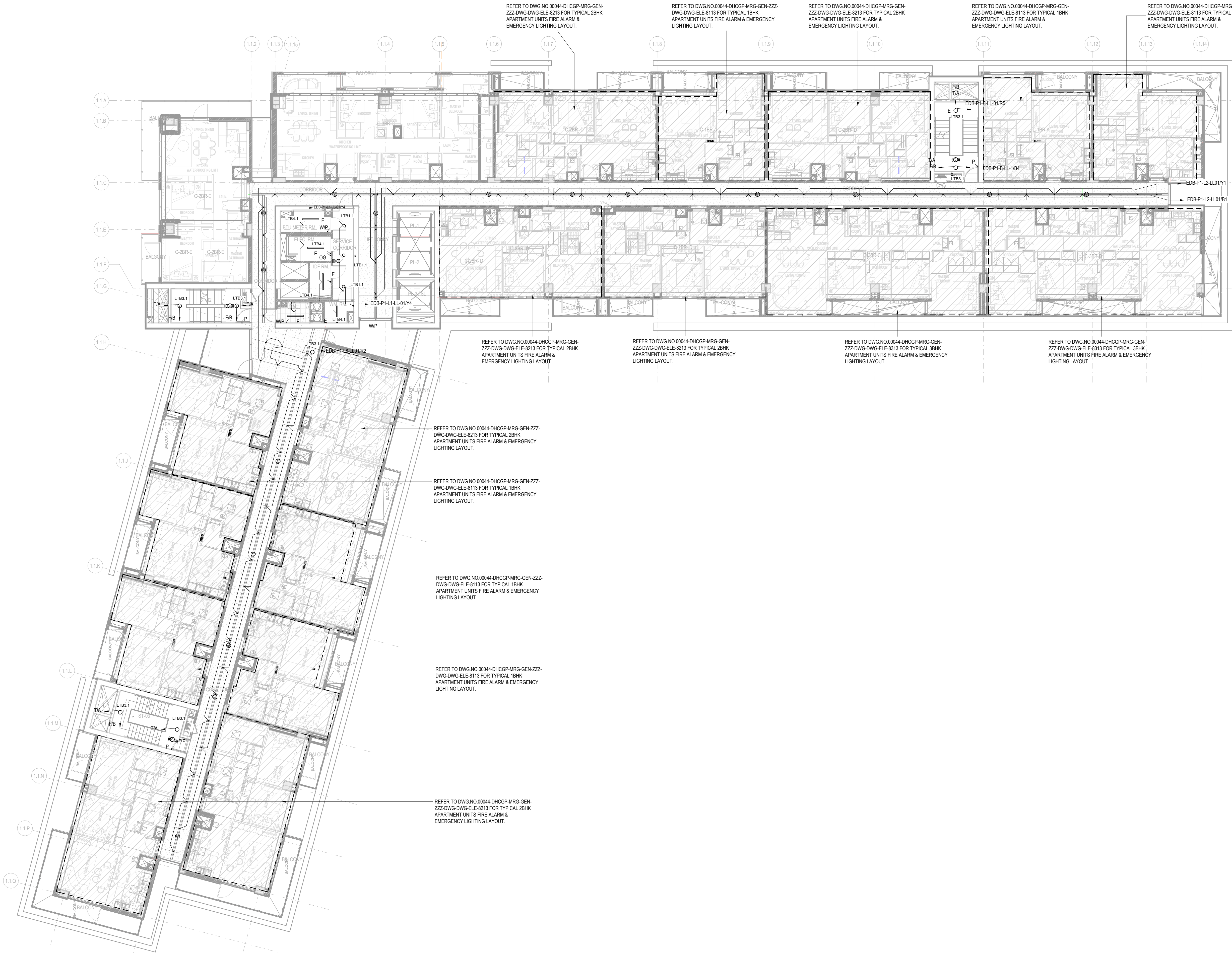
1 BD1-2ND FLOOR (TYP. 3RD TO 6TH FLR.)LIGHTING LAYOUT 1102 1 : 150
